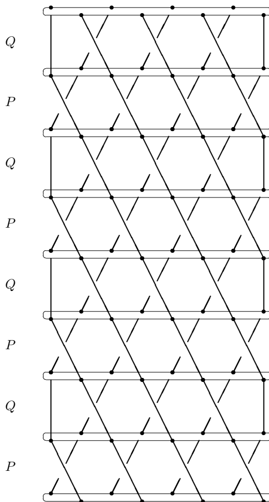
FIGURE 1. The element S in B(6)
