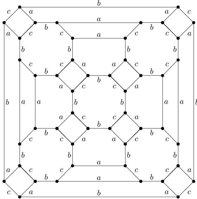
FIGURE 2. The Rhombitruncated Cuboctahedron
